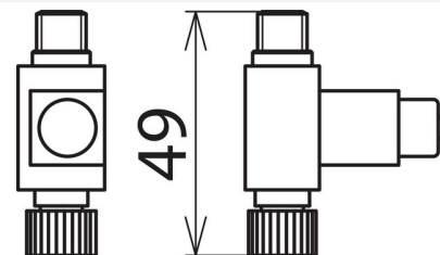
Dimension drawing DGA GF TV
